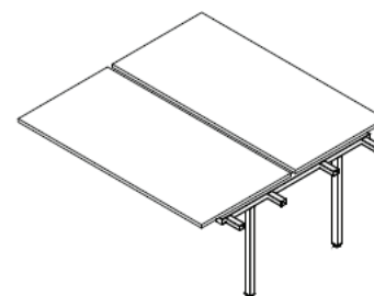
Additional module with a recessed leg
